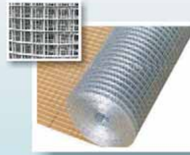
Welded wire meshes Hole dimension - 10x10, 20x20 Raw material - galvanized wire Thickness - 0.6-1.7 mm Width - 1.2 m Max. length - 25 m
