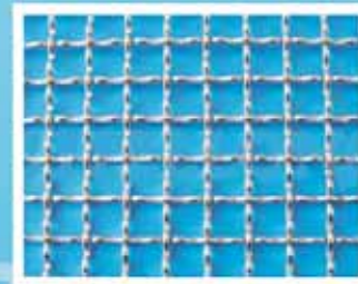
Crimped wire mesh 1000 mm x 2000 mm Hole diameter 20 mm - 200 mm Thickness 3.0 mm - 5.0 mm
